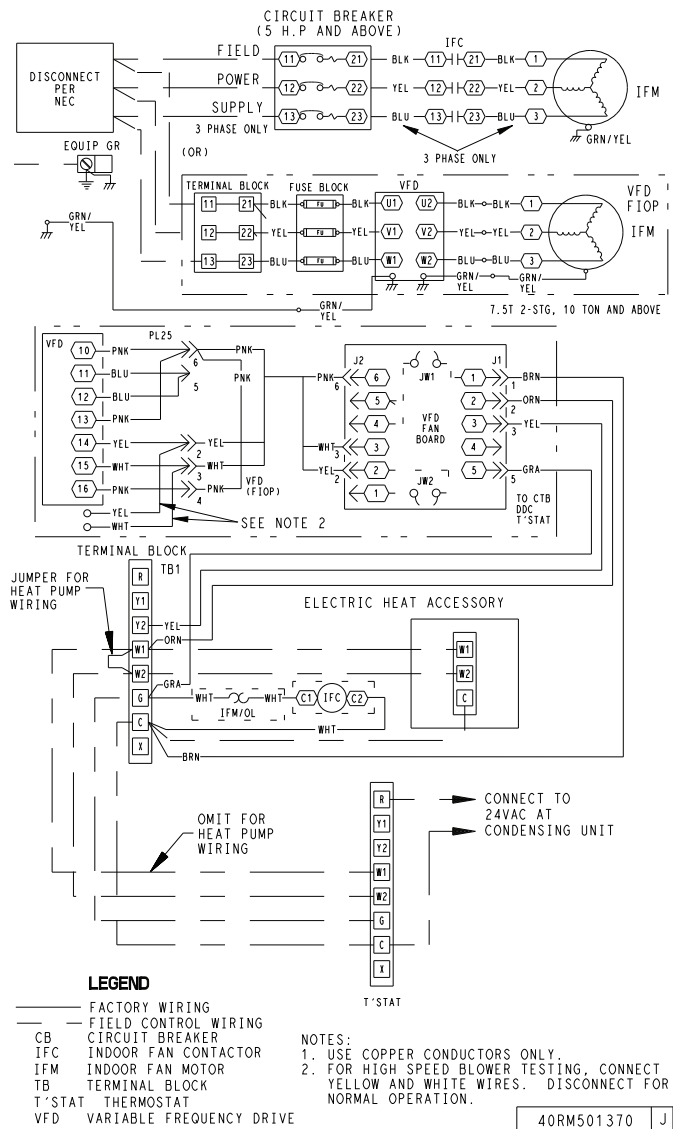
Fig. 37 — Typical Wiring Diagram - Split System Air-Handling Unit (40RU with ACH550 VFD shown)
